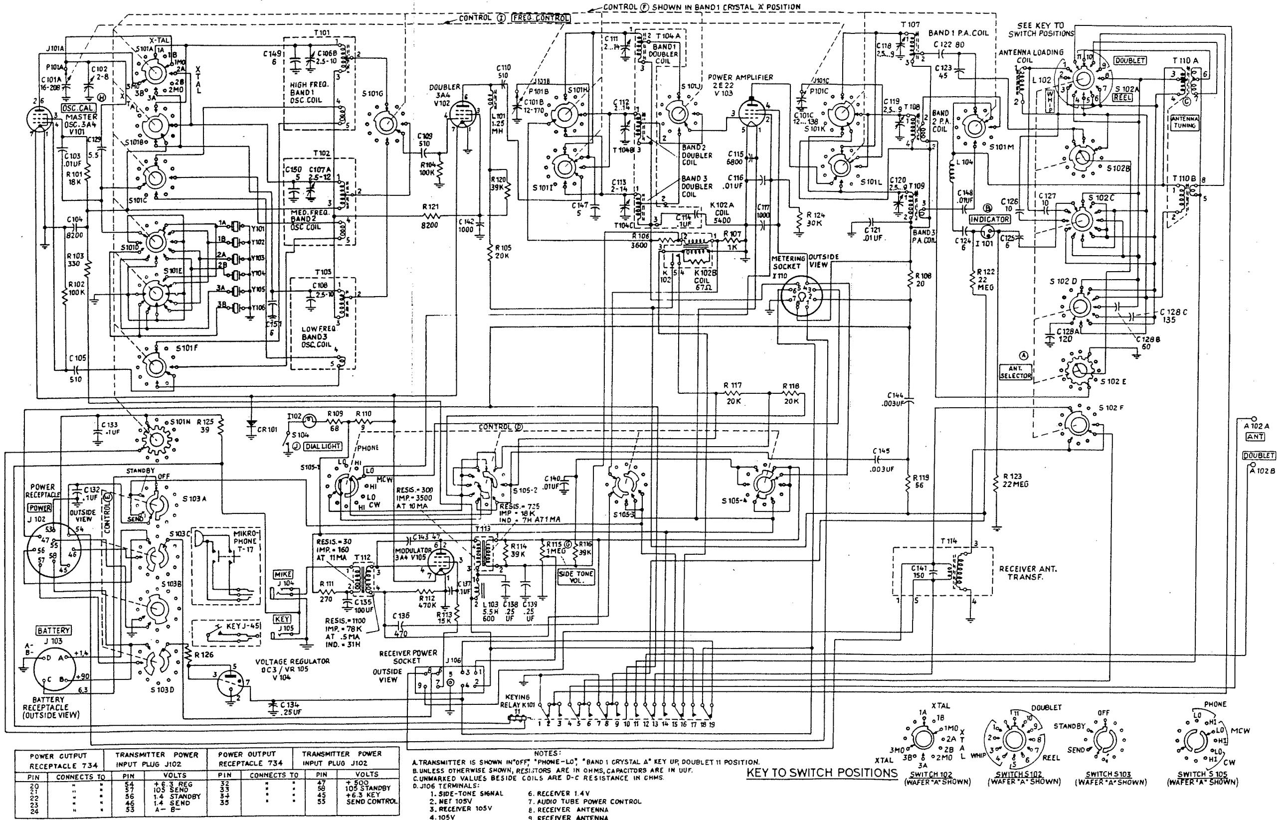
Figure 126 Transmitter section of receiver-transmitter RT-77/GRC-9-6Y, schematic diagram.
